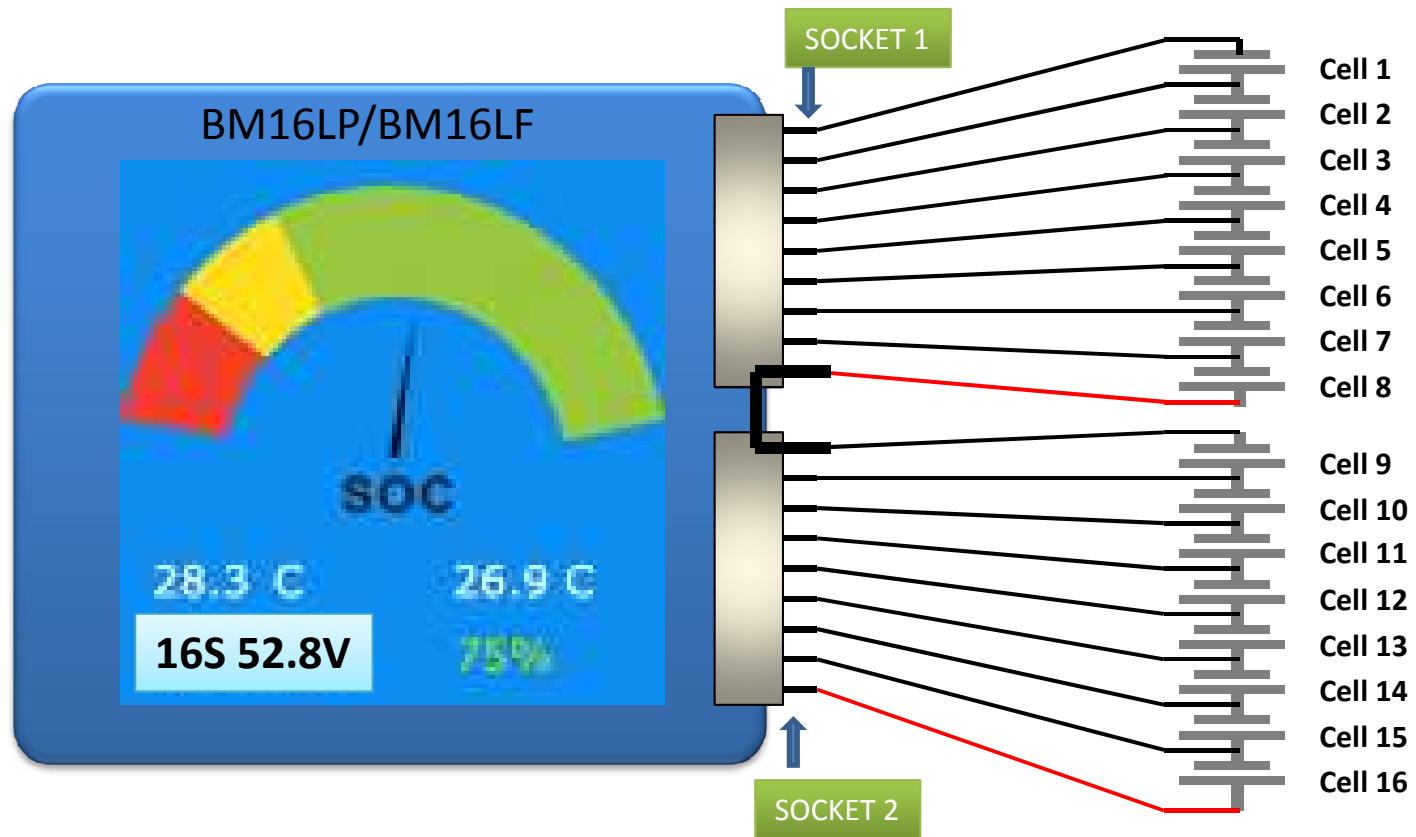
BM16 Connection diagram for two 8S connection in series LiPo/liFe battery pack
